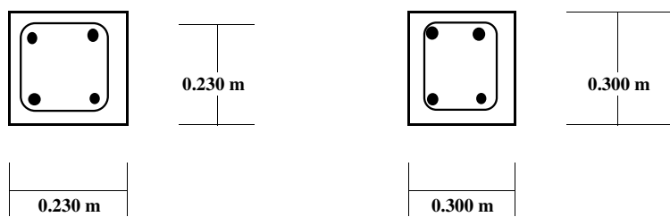
Plan P2
