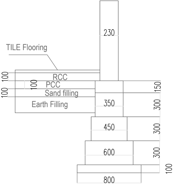
TYP. Section of 230mm thk. Brick Masonry
