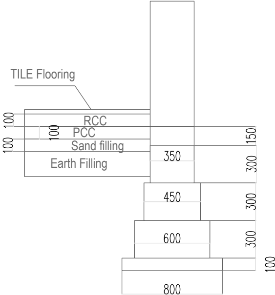
TYP. Section of 350mm thk. Brick Masonry
