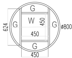
TYP. Drawing of window in 800mm Dia hole with Aluminum Sections.
