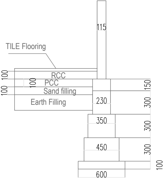
TYP. Section of 115mm thk. Brick Masonry
