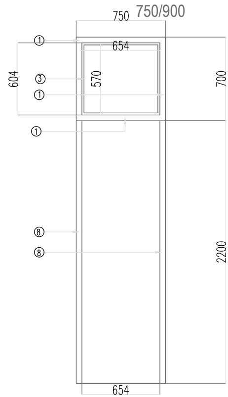
TYP. Drawing of Door with Aluminum Sections.
