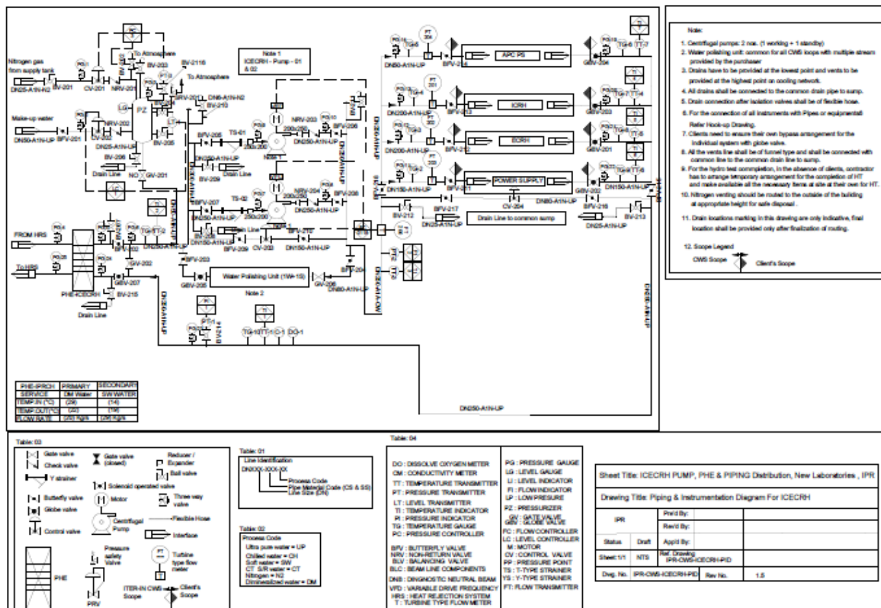
Annexure 27 : ICECRH PID
