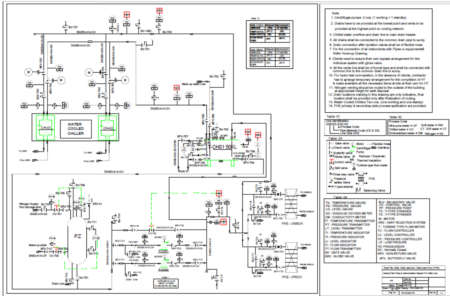
Annexure 32: CHILLER PID
