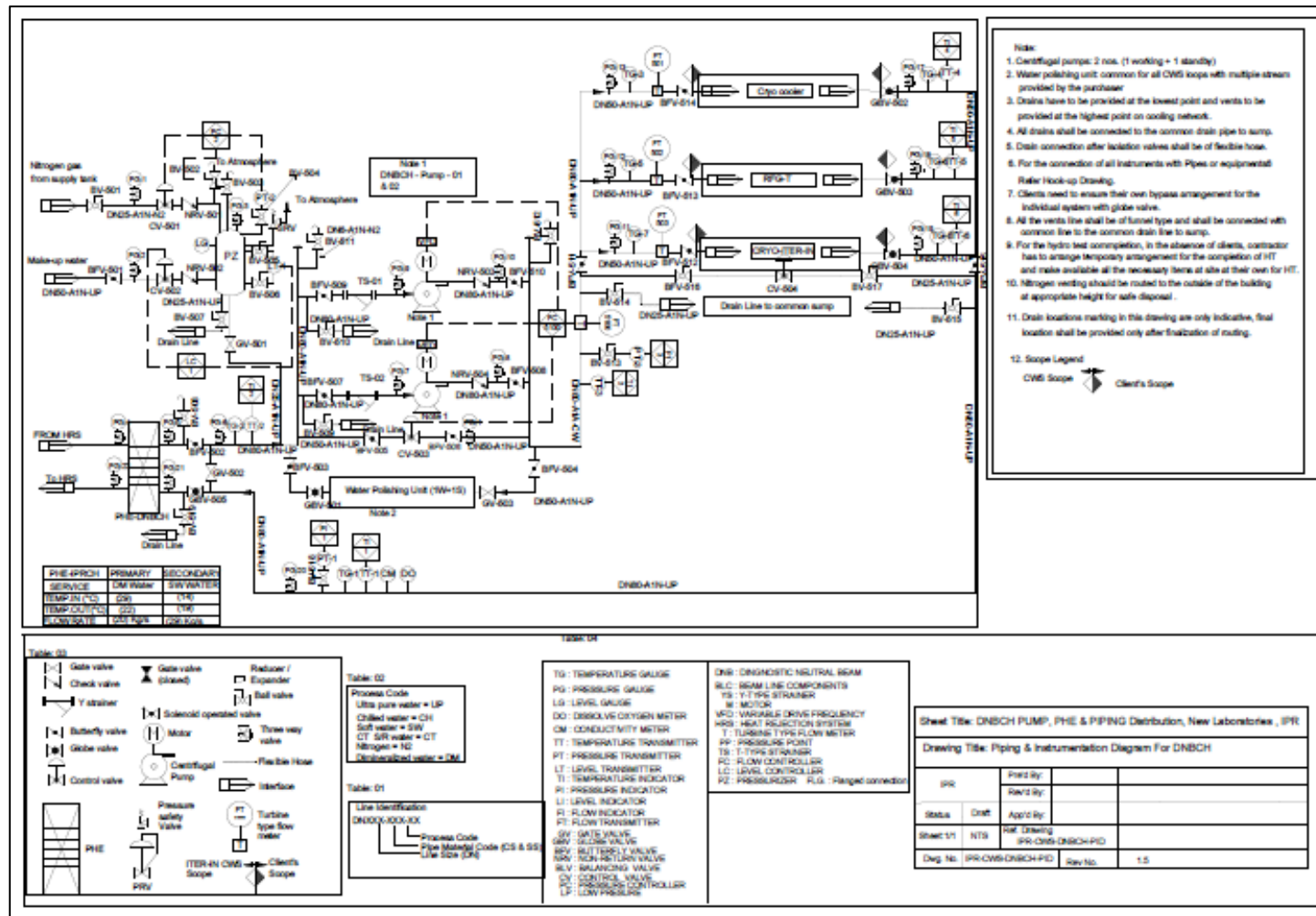
Annexure 30: DNBCH PID
