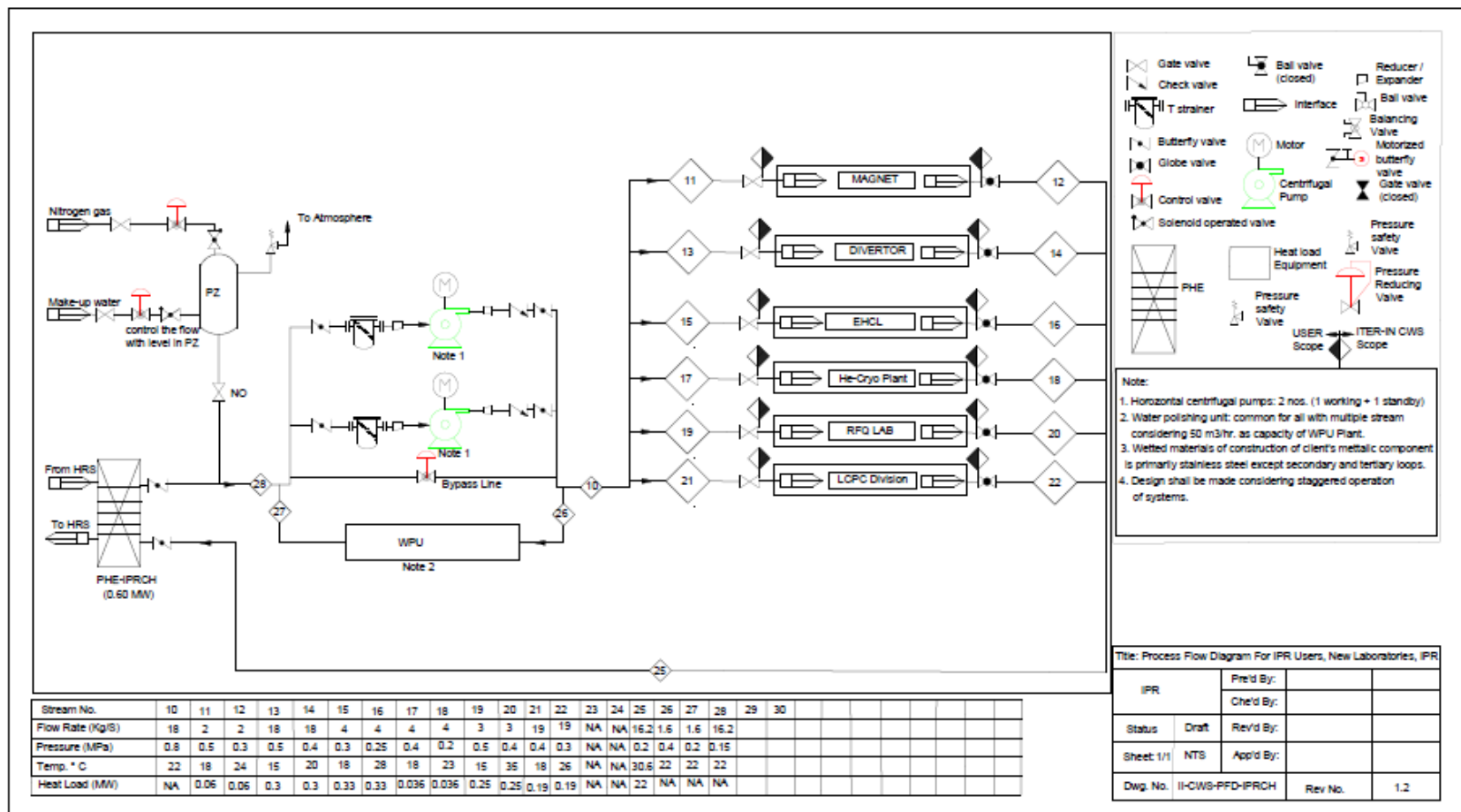
Annexure 25: IPRCH PFD
